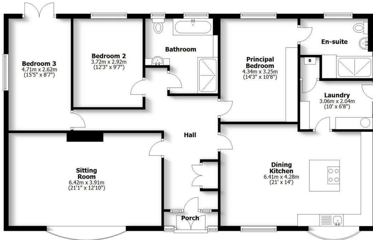
Ground Floor
