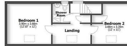
Cottage First Floor
