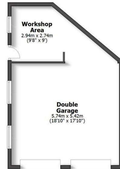
Detached Garage
